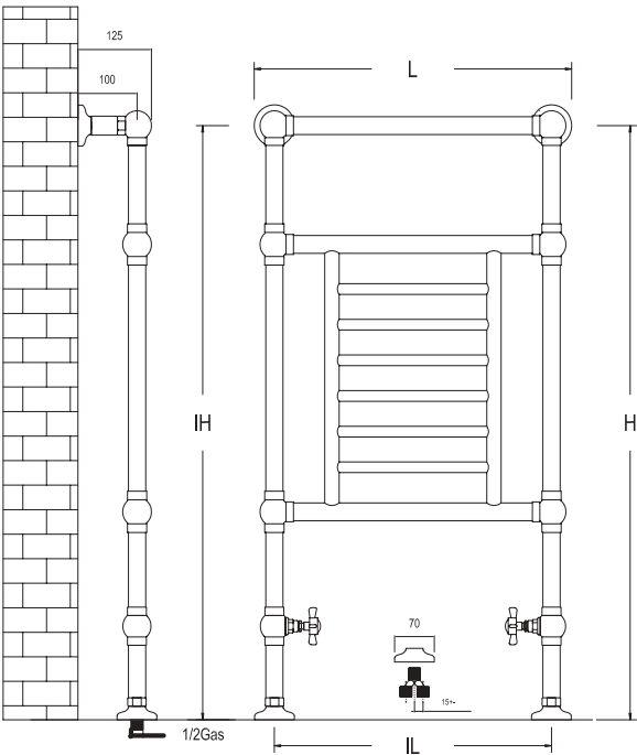
■ SSPV3 • Radiatore a pavimento 3 barre (diverse dimensioni disponibili) Radiateur de sol 3 barres (plusieurs dimensions disponibles) Floor mounted radiator with 3 rails (several sizes available)
