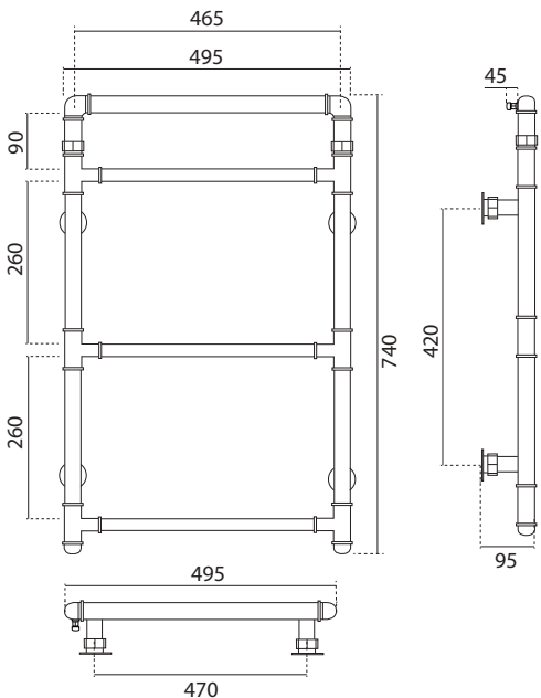
■ SSPMT4 • Radiatore a muro METROPOLITAN 4 barre mm.740x495 250 Kcal/h Radiateur mural METROPOLITAN 4 barres mm.740x495-250 Kcal/h Wall mounted METROPOLITAN radiator with 4 rails mm.740x495-250 Kcal/h
