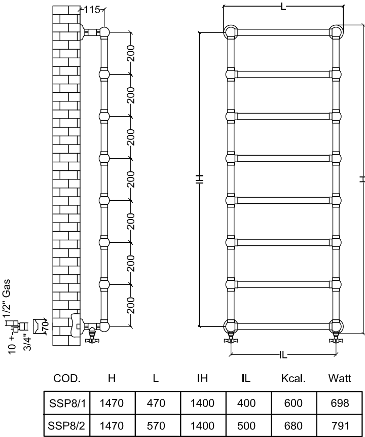
SSP8 • Radiatore a parete 8 barre (diverse dimensioni disponibili) Radiateur mural 8 barres (plusieurs dimensions disponibles) Wall mounted radiator with 8 rails (several sizes available)
