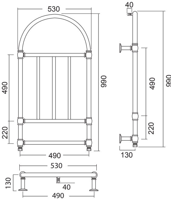
■ SSARC1 • Radiatore a muro ad arco con griglia mm.990x530 DT60° 422 Kcal/h - 481 Watt Radiateur mural arc avec grille mm.990x530 DT60° 422 Kcal/h - 481 Watt Wall mounted arch radiator with grid mm.990x530 DT60° 422 Kcal/h - 481 Watt
