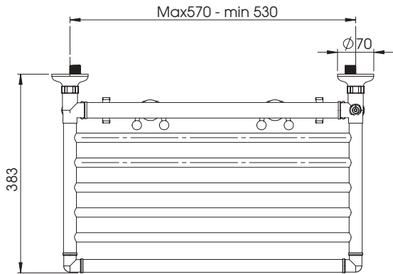
SSCAP1 • Radiatore porta salviette DT60° Kcal/h 293.8 - Watt 340 Radiateur mural porte serviettes DT60° Kcal/h 293.8 - Watt 340 Wall mounted towel holder radiator DT60° Kcal/h 293.8 - Watt 340
