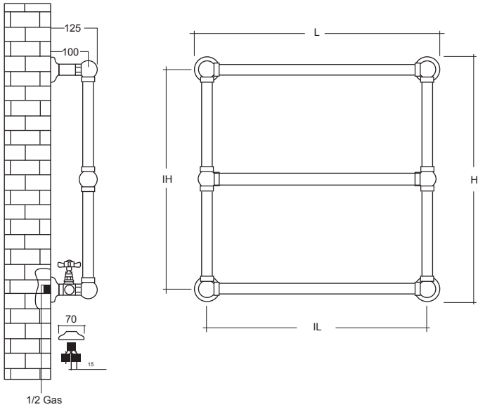
■ SSP3 • Radiatore a parete 3 barre (diverse dimensioni disponibili) Radiateur mural 3 barres (plusieurs dimensions disponibles) Wall mounted radiator with 3 rails (several sizes available)
