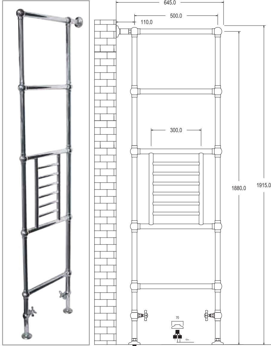
SSPV5DG Radiatore a pavimento 5 barre mm.1915x645 DT60° Kcal/h 706.5 - Watt 819.5 Radiateur de sol 5 barres mm.1915x645 DT60° Kcal/h 706.5 - Watt 819.5 Floor mounted radiator with 5 rails mm.1915x645 DT60° Kcal/h 706.5 - Watt 819.5
