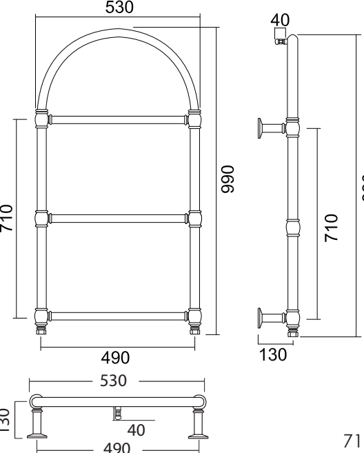
■ SSARC3 • Radiatore a muro ad arco 3 barre mm.990x530 - DT60° 422 Kcal/h - 481 Watts Radiateur Mural arc 3 barres mm.990x530 - DT60° 422 Kcal/h - 481 Watts Wall mounted arc radiator 3 rails mm.990x530 DT60° 422 Kcal/h - 481 Watts
