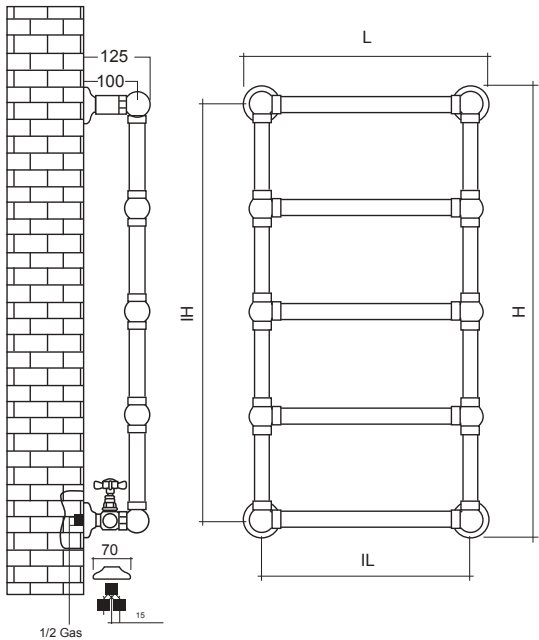
■ SSP5 • Radiatore a parete 5 barre (diverse dimensioni disponibili) Radiateur mural 5 barres (plusieurs dimensions disponibles) Wall mounted radiator with 5 rails (several sizes available)
