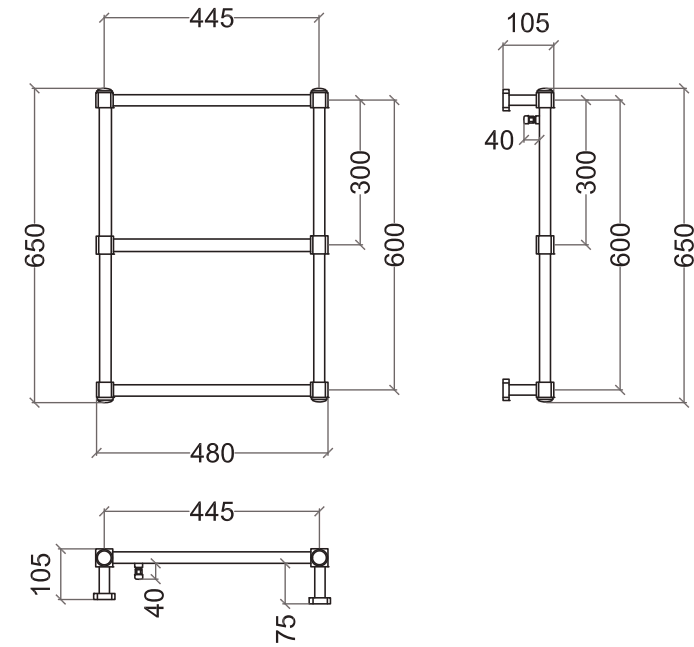
■ SSPTC3 • Radiatore a muro 3 barre mm.650x480 DT60° 274 Kcal/h - 318 Watt Radiateur mural 3 barres mm.650x480 DT60° 274 Kcal/h - 318 Watt Wall mounted radiator with 3 rails mm.650x480 DT60° 274 Kcal/h - 318 Watt
