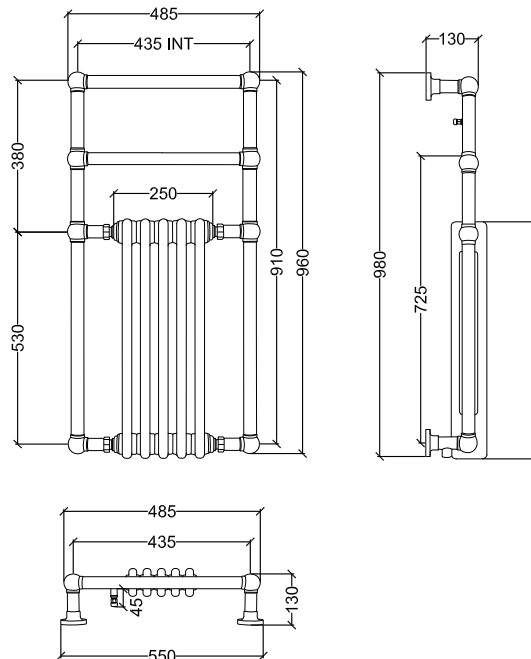
■ SSPINSB4 • Radiatore a muro con inserto in ghisa bianco mm.960x485 DT60° 582Kcal/h - 675 Watt Radiateur mural avec insert en fonte blanche mm.960x485 DT60° 582Kcal/h - 675 Watt Wall mounted radiator with white cast iron insert mm.960x485 DT60° 582Kcal/h - 675 Watt
