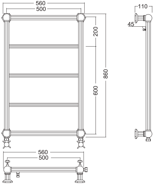
■ SSPLUX5 • Radiatore a muro 5 barre mm.860x560 DT60° 350 Kcal/h - 406 Watt Radiateur mural 5 barres mm.860x560 DT60° 350 Kcal/h - 406 Watt Wall mounted radiator with 5 rails mm.860x560 DT60° 350 Kcal/h - 406 Watt
