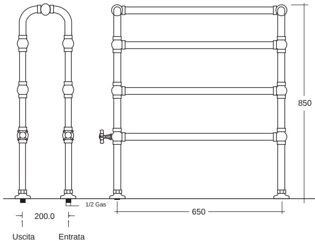
■ SSCA7CR • Radiatore a cavalletto da pavimento a cromo DT60° Kcal/h 762 - Watt 884 Radiateur chevalet de sol chromé DT60° Kcal/h 762 - Watt 884 Floor mounted easel radiator chrome DT60° Kcal/h 762 - Watt 884
