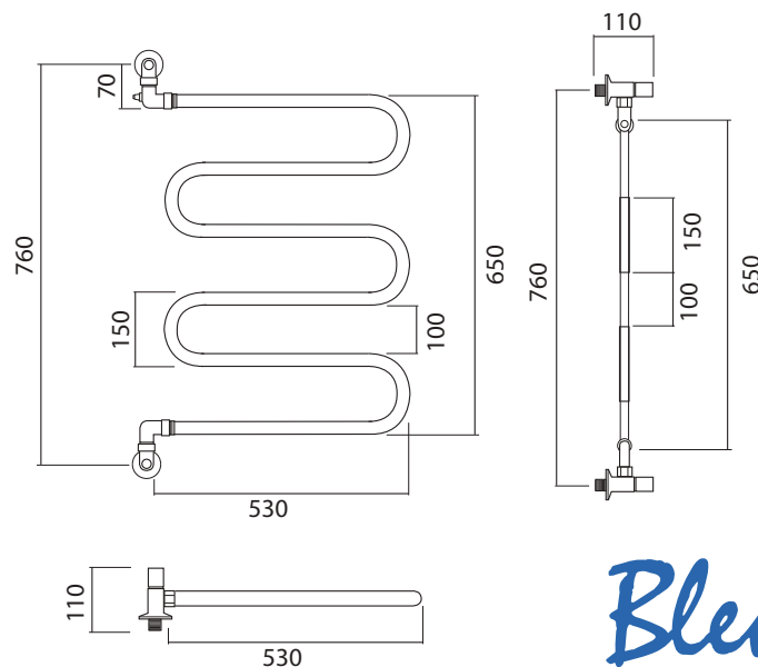
■ SSERP6CR • Radiatore a muro serpentina 6 barre cromo mm.760x650 DT60° 160 Kcal/h - 185 Watt Radiateur mural serpentin 6 barres chromé mm.760x650 DT60° 160 Kcal/h - 185 Watt Wall mounted radiator with 6 rails chrome mm.760x650 DT60° 160 Kcal/h - 185 Watt
