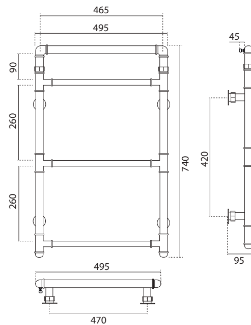
■ SSPMT4BR • Radiatore a muro METROPOLITAN 4 barre bronzo mm.495x740 250 Kcal/h Radiateur mural METROPOLITAN 4 barres bronze mm.495x740-250 Kcal/h Wall mounted METROPOLITAN radiator with 4 rails bronze mm.495x740-250 Kcal/h
