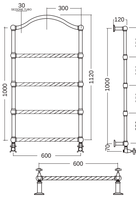
■ SSARC2OR • Radiatore a muro ad arco 5 barre oro mm.1000x600 DT60° 530 Kcal/h - 615 Watt Radiateur mural arc 5 barres or mm.1000x600 DT60° 530 Kcal/h - 615 Watt Wall mounted arch radiator with 5 rails gold mm.1000x600 DT60° 530 Kcal/h - 615 Watt
