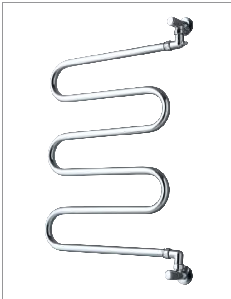
■ SSERP6CR • Radiatore a muro serpentina 6 barre cromo mm.760x650 DT60° 160 Kcal/h - 185 Watt Radiateur mural serpentin 6 barres chromé mm.760x650 DT60° 160 Kcal/h - 185 Watt Wall mounted radiator with 6 rails chrome mm.760x650 DT60° 160 Kcal/h - 185 Watt
