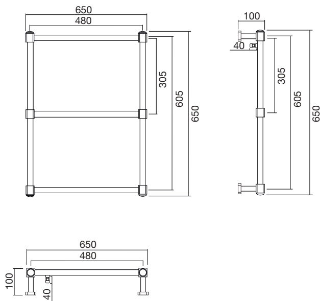
■ SSPTC3CR • Radiatore a muro 3 barre cromo mm.650x650 DT60° 274 Kcal/h - 318 Watt Radiateur mural 3 barres chromé mm.650x650 DT60° 274 Kcal/h - 318 Watt Wall mounted radiator with 3 rails chrome mm.650x650 DT60° 274 Kcal/h - 318 Watt
