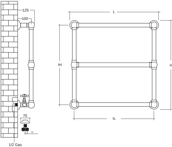
■ SSP3CR • Radiatore a parete 3 barre cromo (diverse dimensioni disponibili) Radiateur mural 3 barres chromé (plusieurs dimensions disponibles) Wall mounted radiator with 3 rails chrome (several sizes available)
